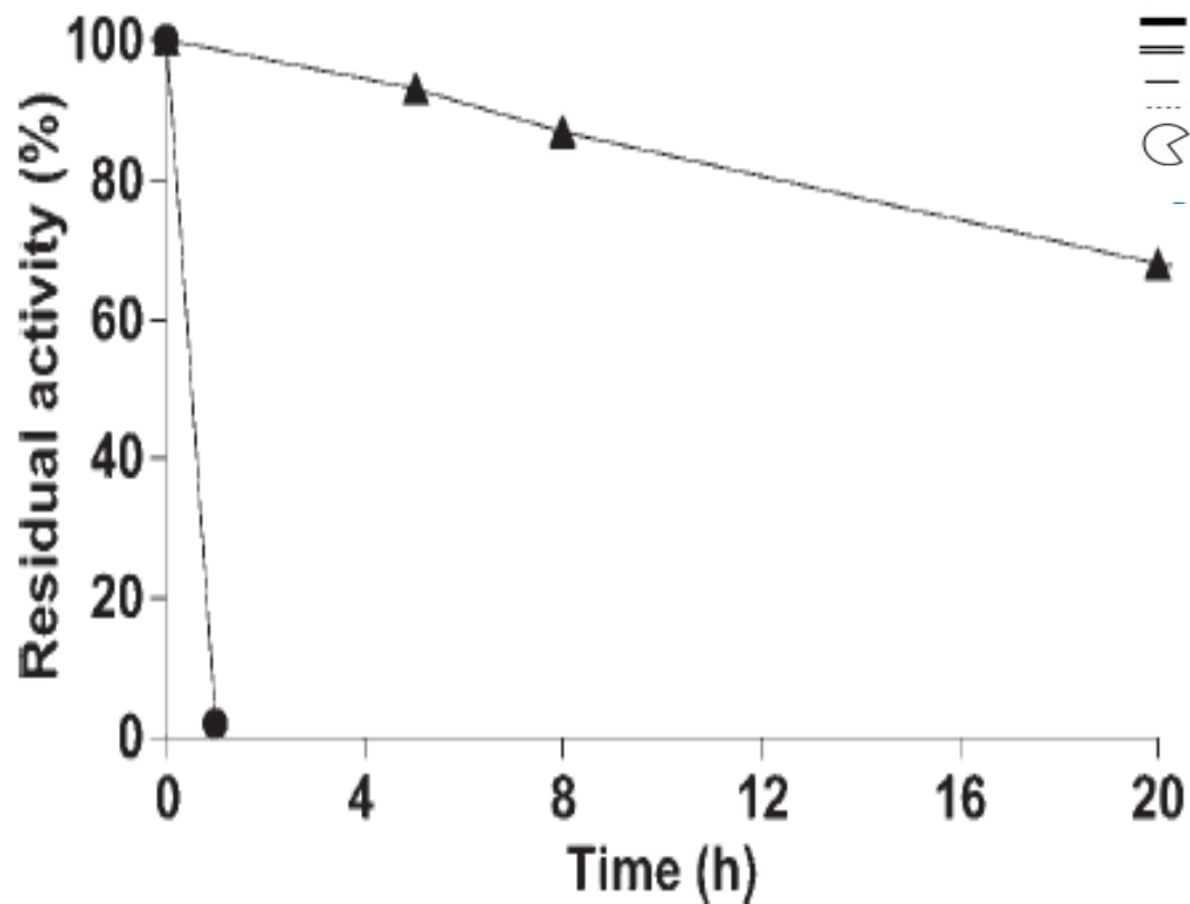
Fig. 4. Thermal stability of different GOX preparations. Triangle, immobilized on MANAE agarose activated with glutaraldehyde. Circle, soluble enzyme. Inactivation conditions were 56°C, pH 7.0, and 0.4 U/mL.
