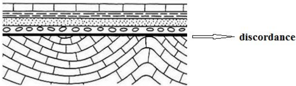
Fig.23 Discordance angulaire
