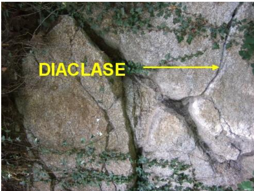
Fig 27 Diaclase
