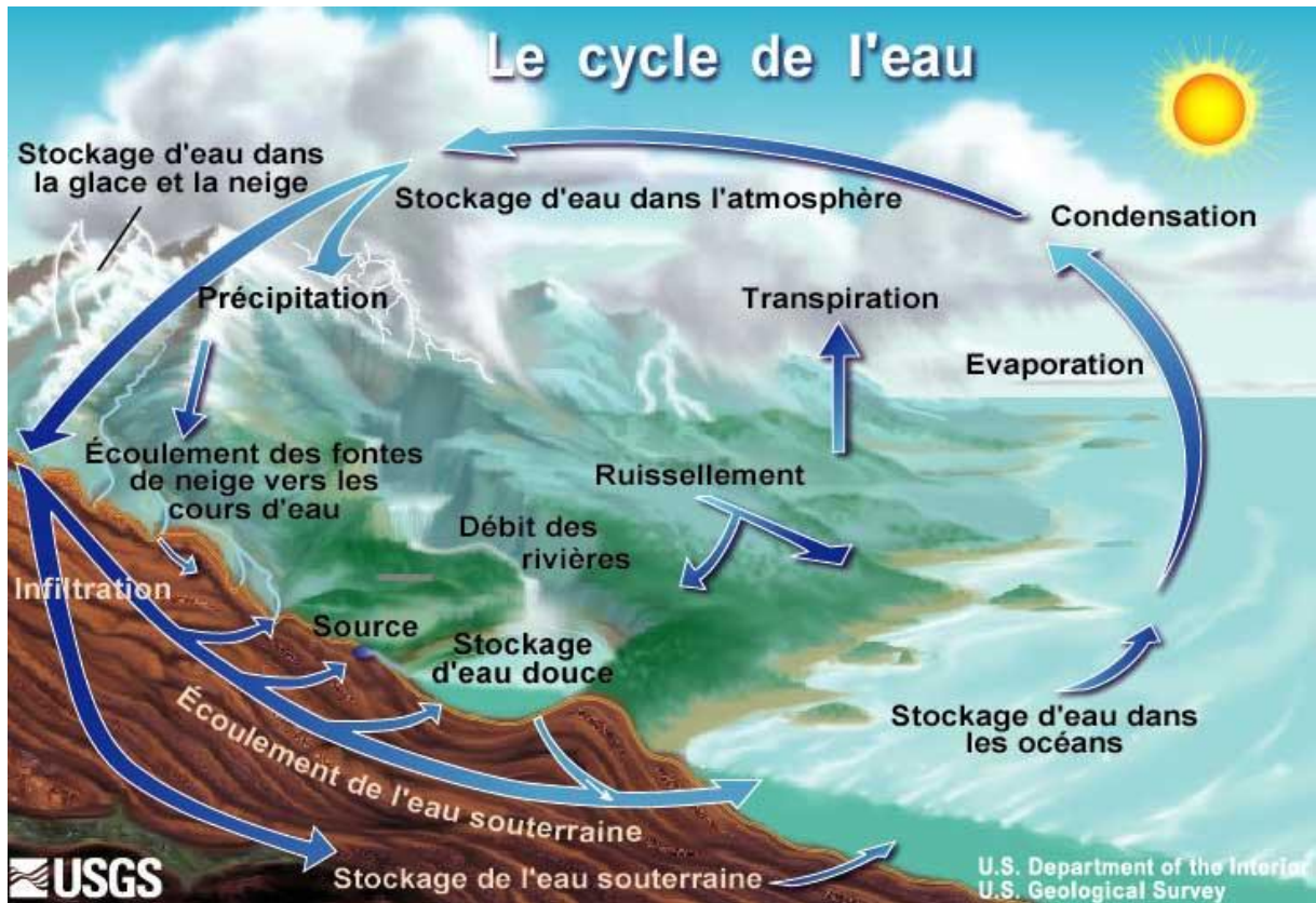
Fig. 4 : le cycle de l'eau (US. Department of the interior, US. Geological Survey)
