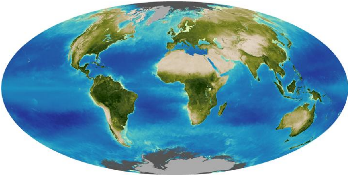
Fig. 3 biosphere(earthobservatory.nasa.gov)
