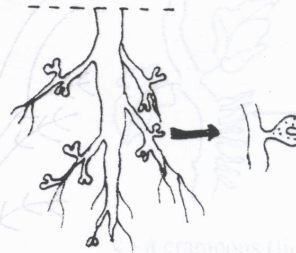
Figure 6: mycorhizes (racine + champignon).
